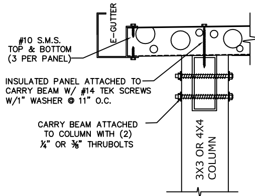
INSULATED PANEL, BEAM & COLUMN ATTACHMENT 2
