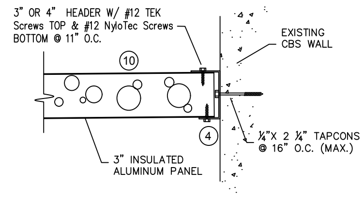
INSULATED PANEL TO CBS WALL
