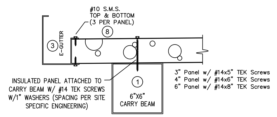
INSULATED PANEL TO BEAM ATTACHMENT
