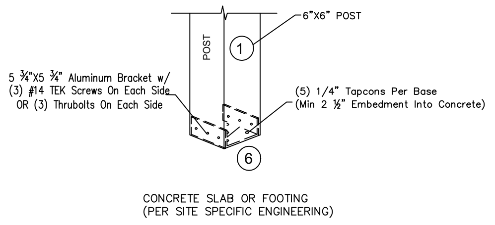
POST ATTACHMENT OVER CONCRETE (ATTACHED)
