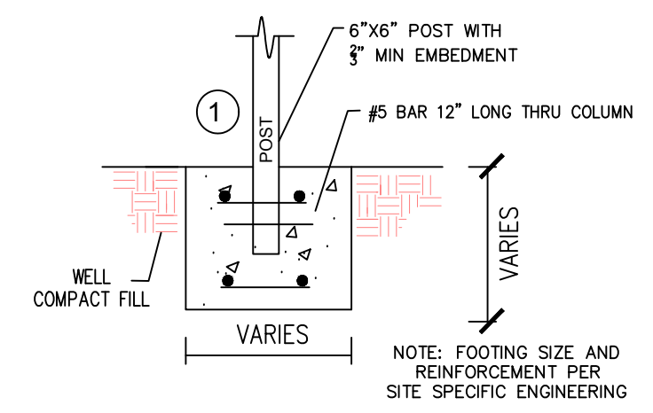
POST ATTACHMENT (FREESTANDING)
