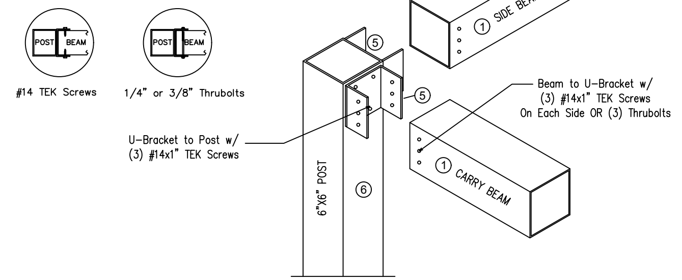
POST TO BEAM CONNECTION
