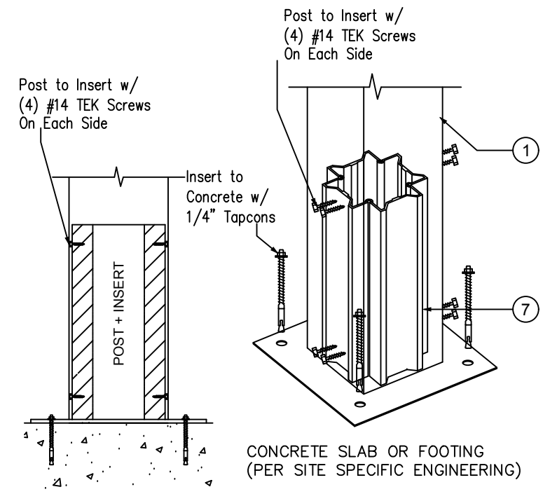
POST ATTACHMENT (INSERT)
