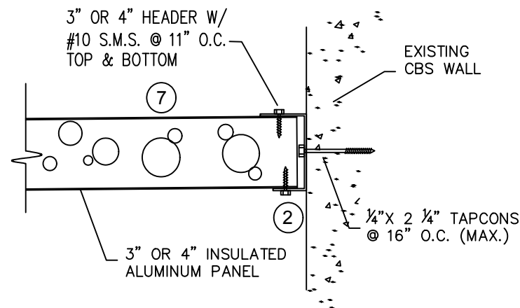
INSULATED PANEL TO CBS WALL
