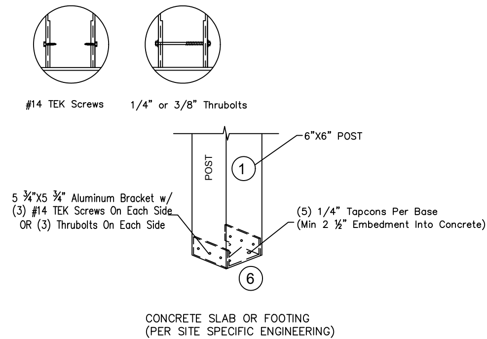
POST ATTACHMENT OVER CONCRETE (ATTACHED)
