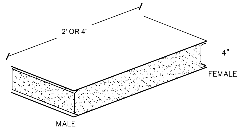
4" Insulated Aluminum Panel
