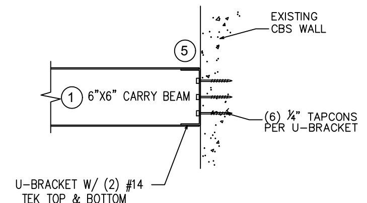
BEAM TO CBS WALL CONNECTION
