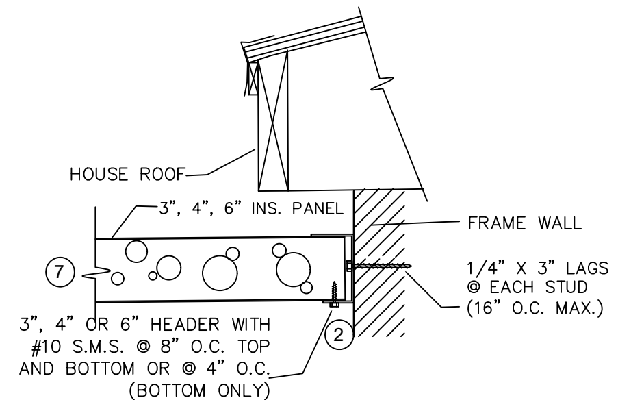
INSULATED PANEL TO FRAME WALL
