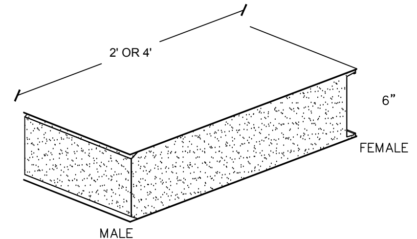
6" Insulated Aluminum Panel
