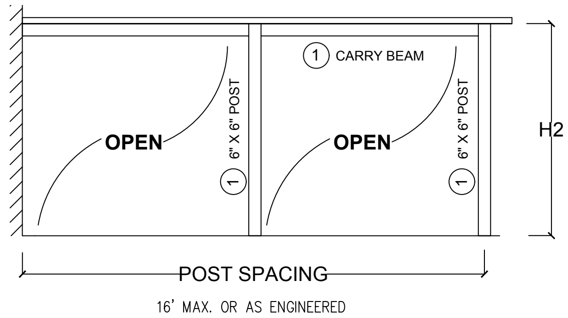
L- SHAPE ATTACHEMENT
