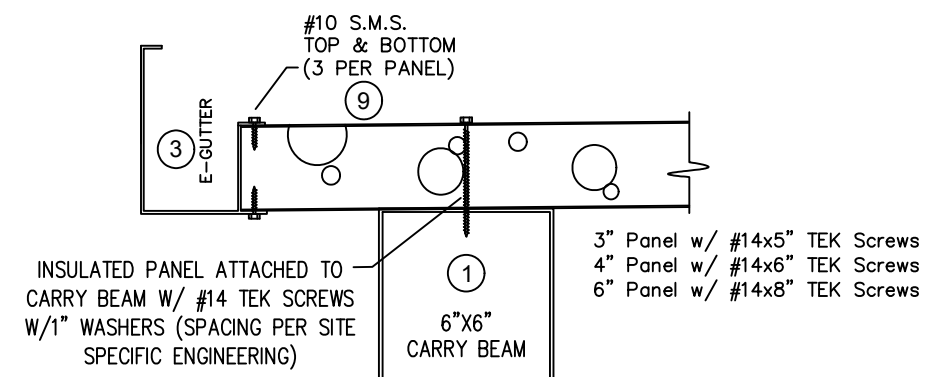
INSULATED PANEL TO BEAM ATTACHMENT
