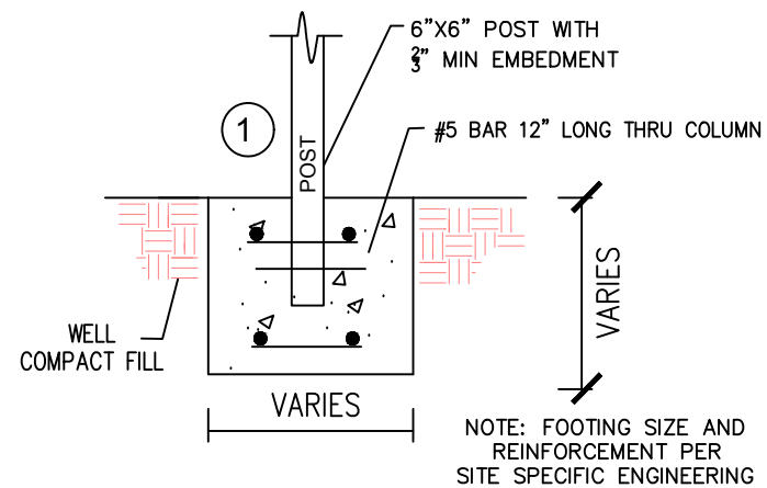
POST ATTACHMENT (FREESTANDING)
