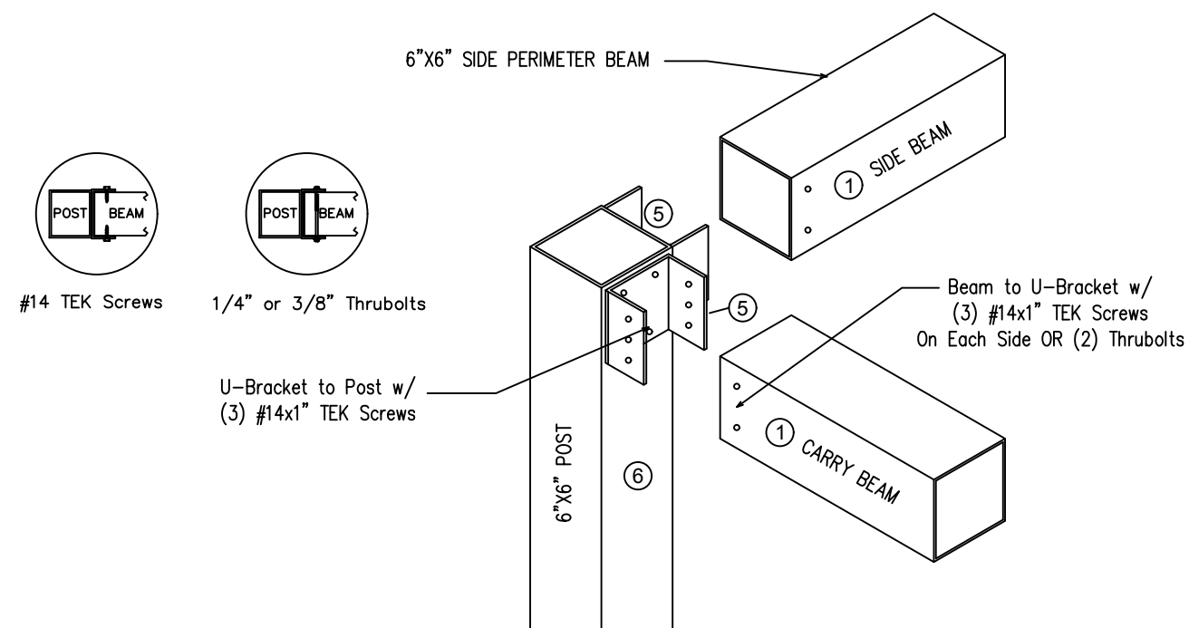
POST TO BEAM CONNECTION
