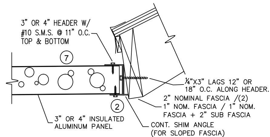
INSULATED PANEL TO FASCIA
